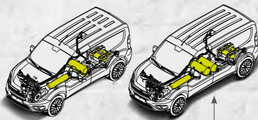
CARGO MAXI VERSION WITH ADDITIONAL METHANE TANK (OPT. 422)
